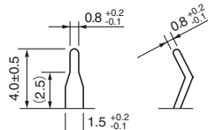
(Terminal dimensions)
