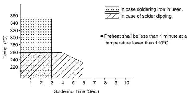
Fig 2 Solder temp. and soldering time
