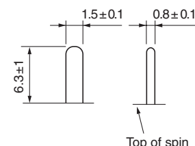
Terminal dimensions
