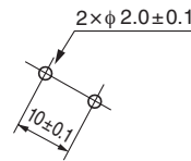
PC board hole dimensions
