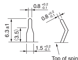
Terminal dimensions
