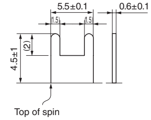
Terminal dimensions
