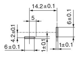
PC board hole dimensions
