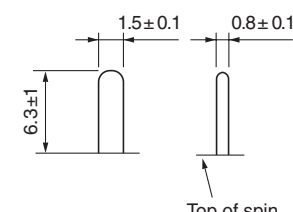
Terminal dimensions
